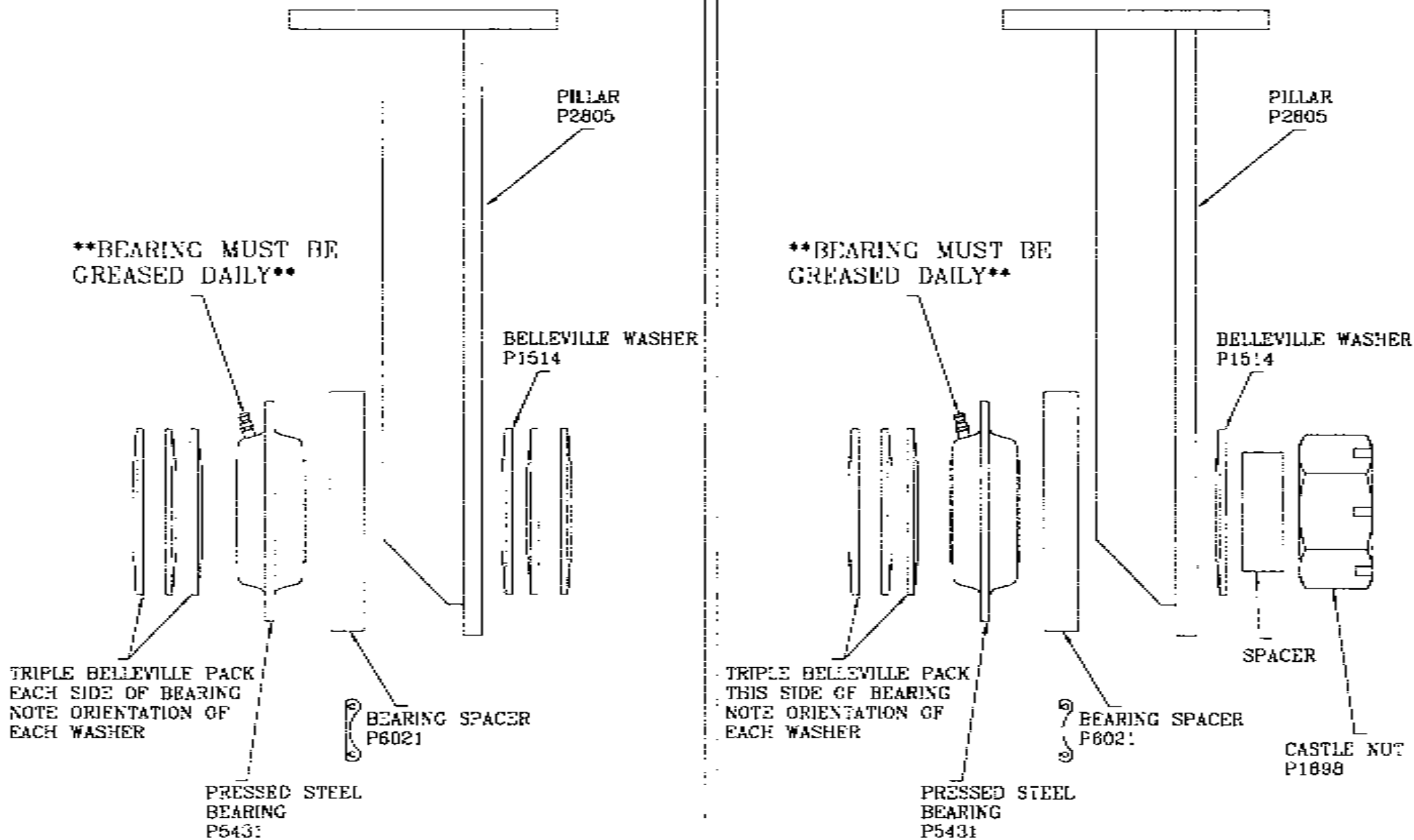
TRIPLE BELLEVILLE PACK - CENTRE PILLAR LAYOUT
