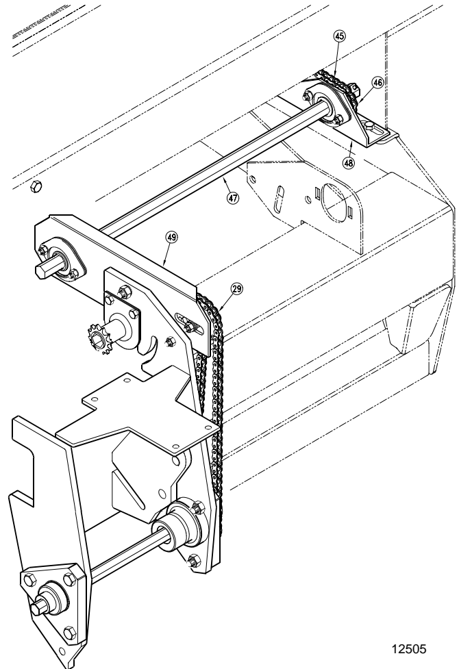
Figure 4 Chain Installation
