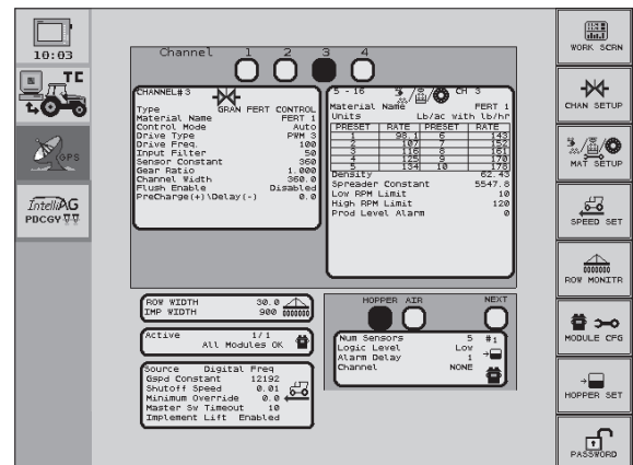
Summary Screen
